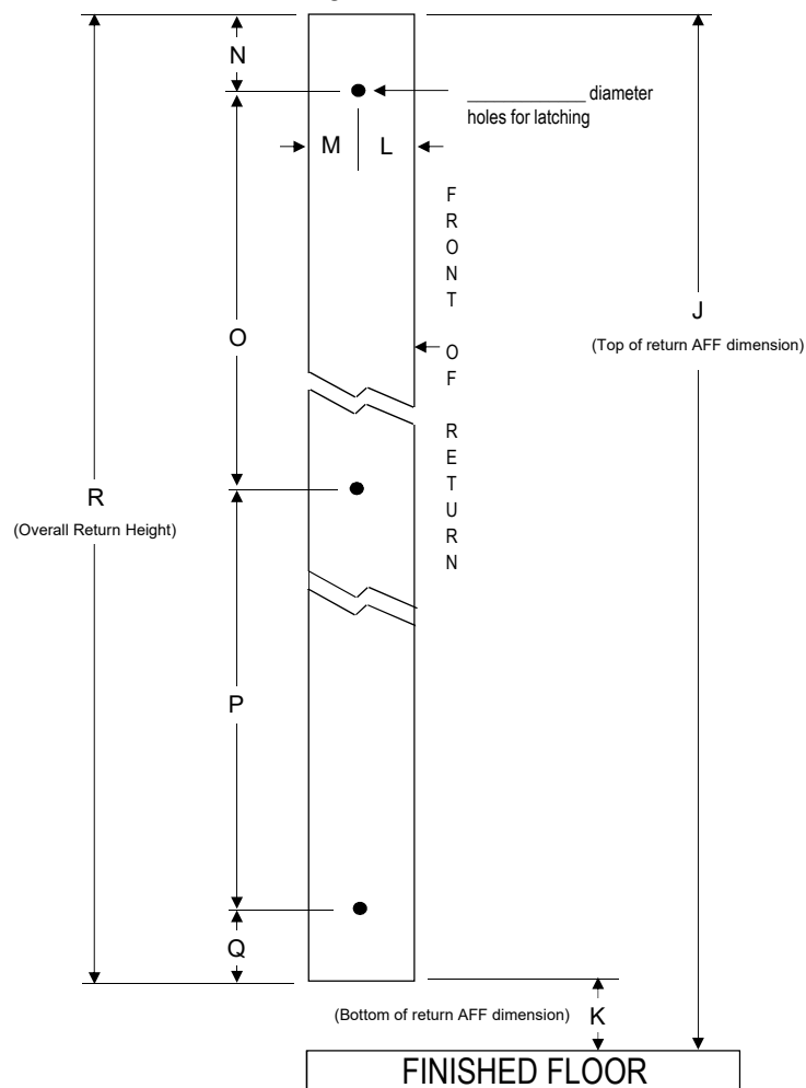
Jamb Side View of Swing Return
