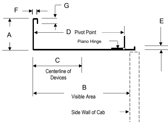
Top View of Swing Return
