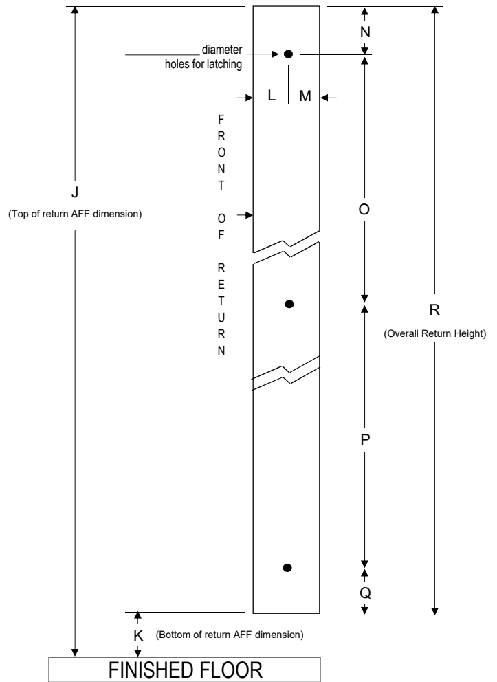
Jamb Side View of Swing Return
